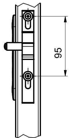
Detail B
