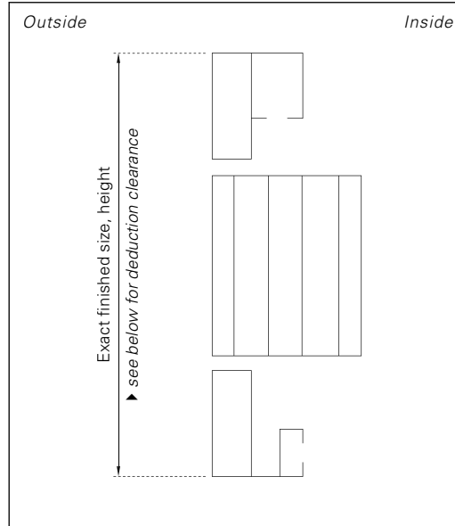
Vertical cross-section
