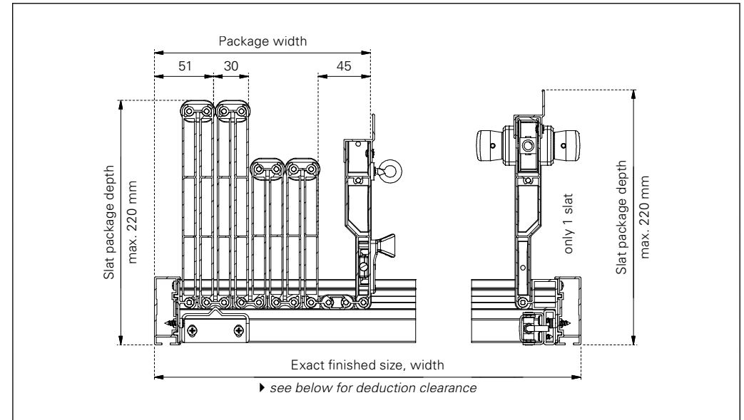
Horizontal cross-section
