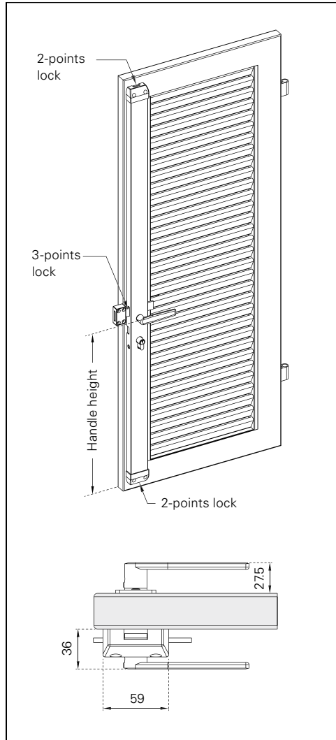
R75 frame
