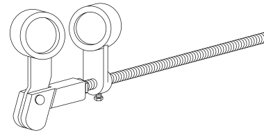
Shutter holder, M10 thread, adjustable, 130 mm
