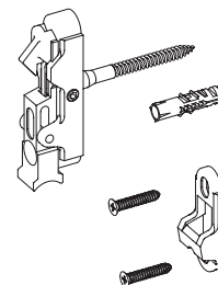
Door shutter holder with carrier screw and dowel,
