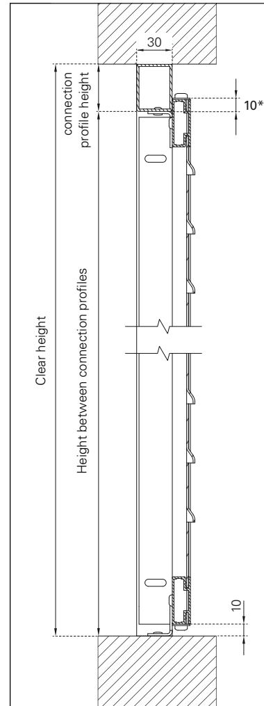
Connection profile only at the top
