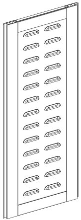
Continuous louvres Louvred panel, 1.5 mm, grid 50 mm, embossed (60×12×6 mm)
