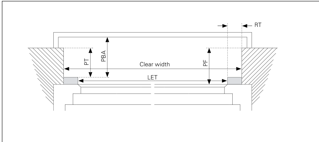
Installation type 1 | Connection profile on the reveal
