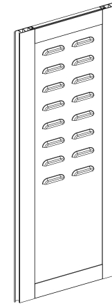
Louvres ⅔ from top Louvred panel, 1.5 mm, grid 50 mm, embossed (60×12×6 mm)
