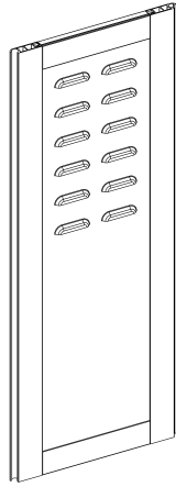
Louvres ½ from top Louvred panel, 1.5 mm, grid 50 mm, embossed (60×12×6 mm)
