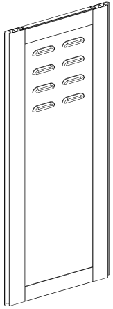
Louvres on the top third Louvred panel, 1.5 mm, grid 50 mm, embossed (60×12×6 mm)
