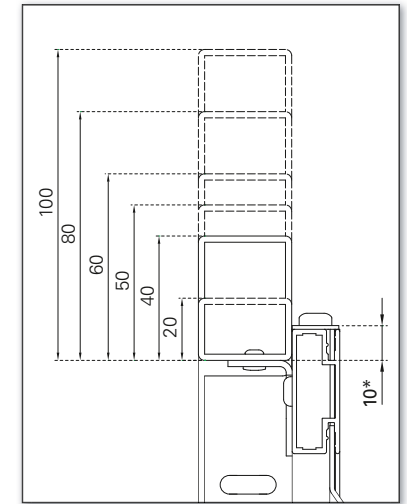
Connection profile heights
