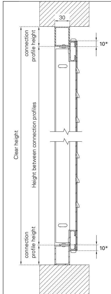
Connection profile at the top and at the bottom
