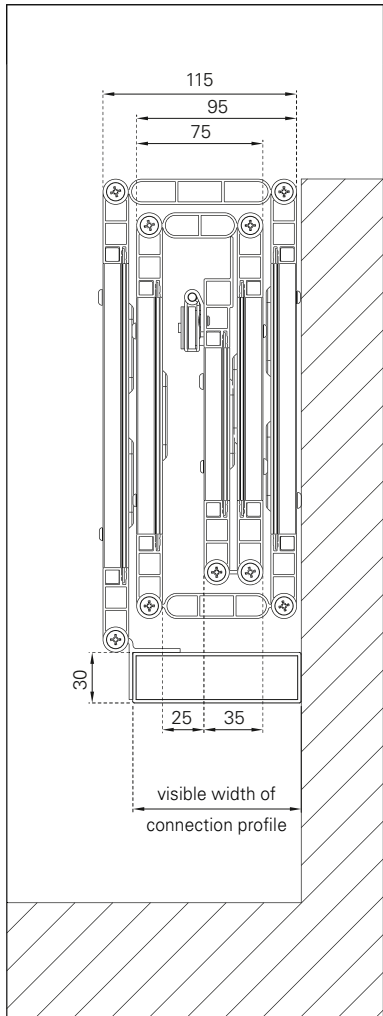
System cross-section
