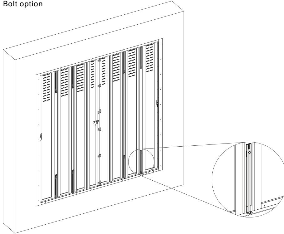
Bolt option
