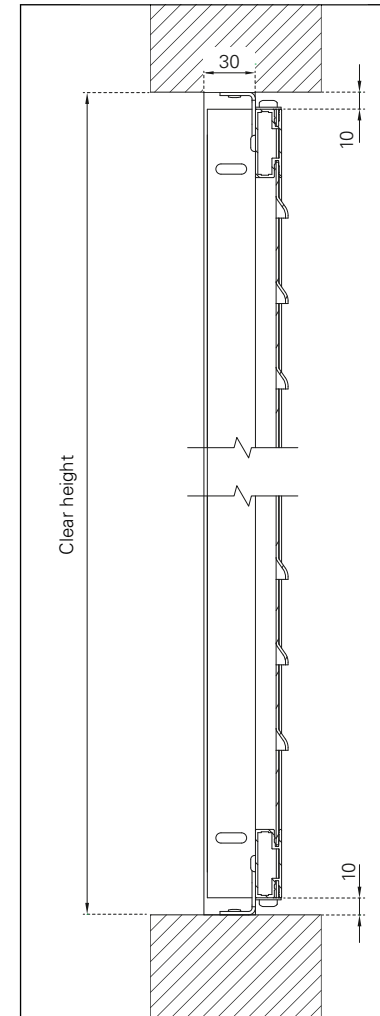
Without connection profile
