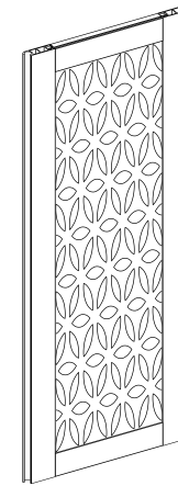
Individual design 1.5 mm sheet metal insert, lasered design cutout (data supplied by the customer)
