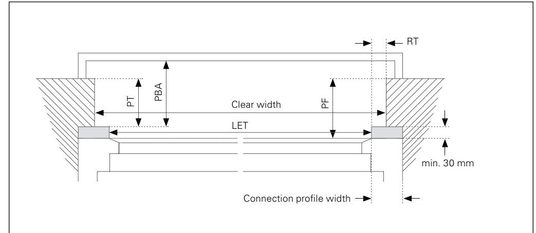
Installation type 2 | Connection profile inset in the masonry
