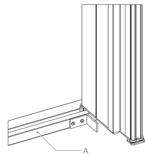
PROVENCE barrier-free
