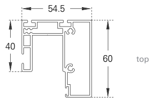
Frame profile
