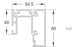
Frame profile
