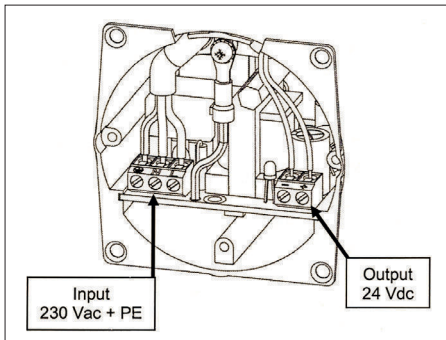
Electrical connection
