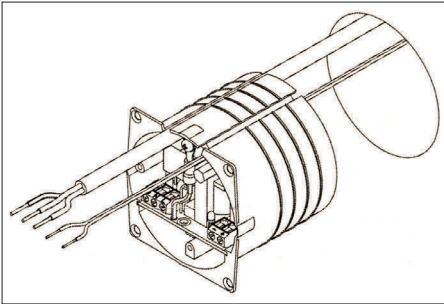
Cable entry
